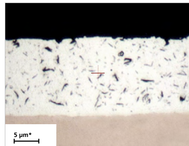
Finely dispersed graphite particles are embedded in the silver layer as shown in the microsection.
